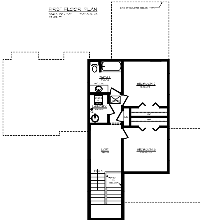
SECOND FLOOR PLAN SCALE: 1/4" = 1'-0" 8'-0" WALL HT. 682 SQ. FT.
