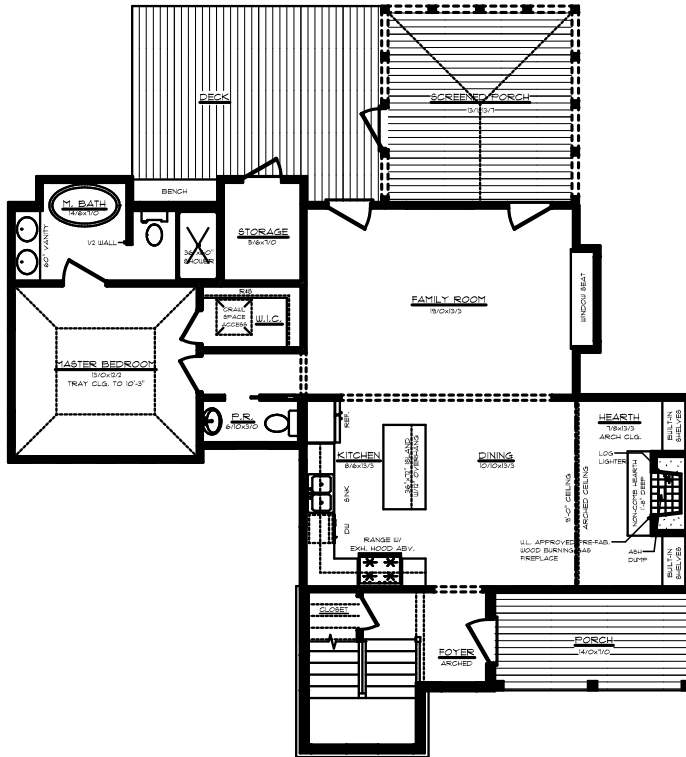
FIRST FLOOR PLAN SCALE: 1/4" = 1'-0" 9'-0" CLG. HT. 122 SQ. FT.
