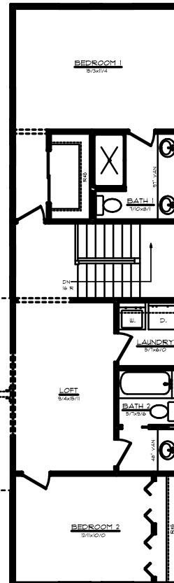
SECOND FLOOR PLAN SCALE: 1/4" = 1'-0" 8'-0" CLG. HT. 1218 SQ. FT. (UNLESS NOTED OTHERWISE)
